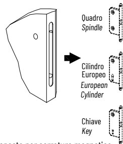
Anta predisposta per serratura magnetica Pre-mortised door (hole) for magnetic lock
