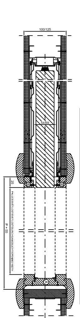
CARTONGESSO - SADROKARTON - SADROKARTON - GIPS-KARTON - PLASTERBOARD
